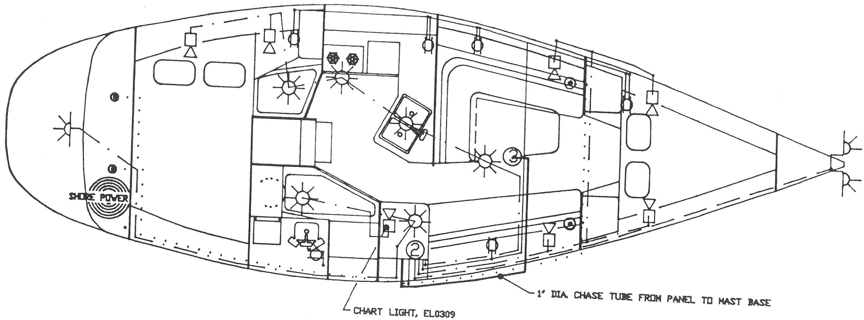
WIRE HARNESS 'A'
