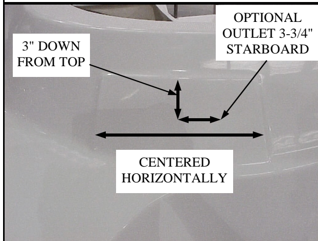
LOCATION OF SHORE POWER OUTLET AND OPTION SECOND OUTLET
