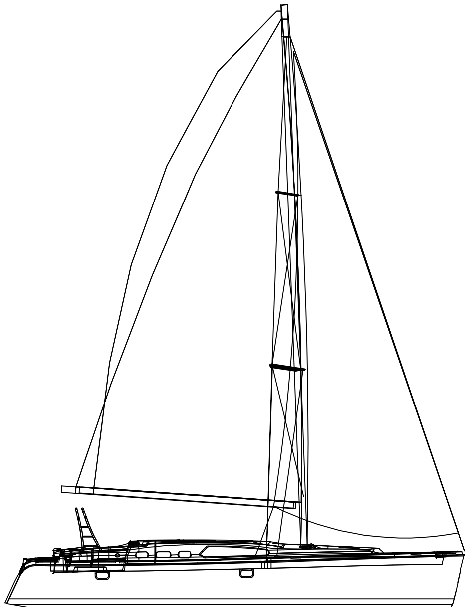
CONFIGURATION 1 OVERLAP JIB NO STAYSAIL JIB SHEETS ON SIDE DECK NO SELF-TACKING
