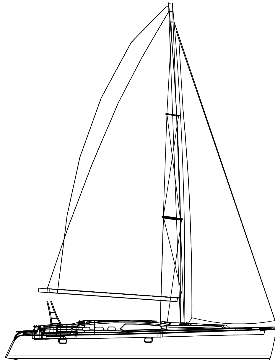
CONFIGURATION 2 NON-OVERLAP JIB NO STAYSAIL JIB SHEETS ON SELF-TACKING APPARATUS
