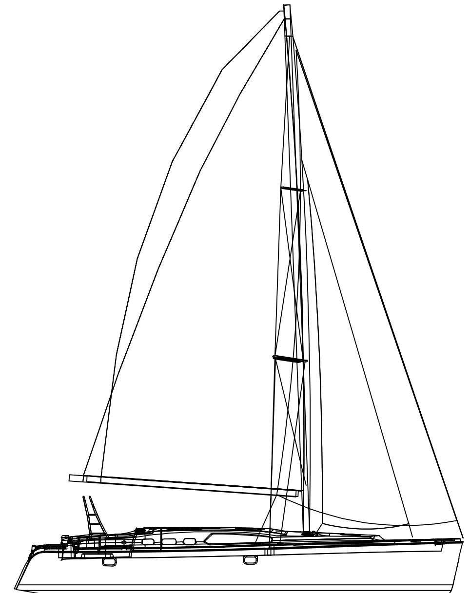
CONFIGURATION 3 OVERLAP JIB STAYSAIL ON SELF-TACKING APPARATUS JIB SHEETS ON SIDE DECK
