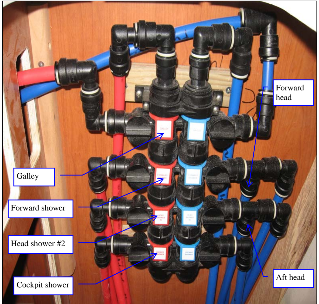
The picture shows waterline arrangement on the brand new water manifold
